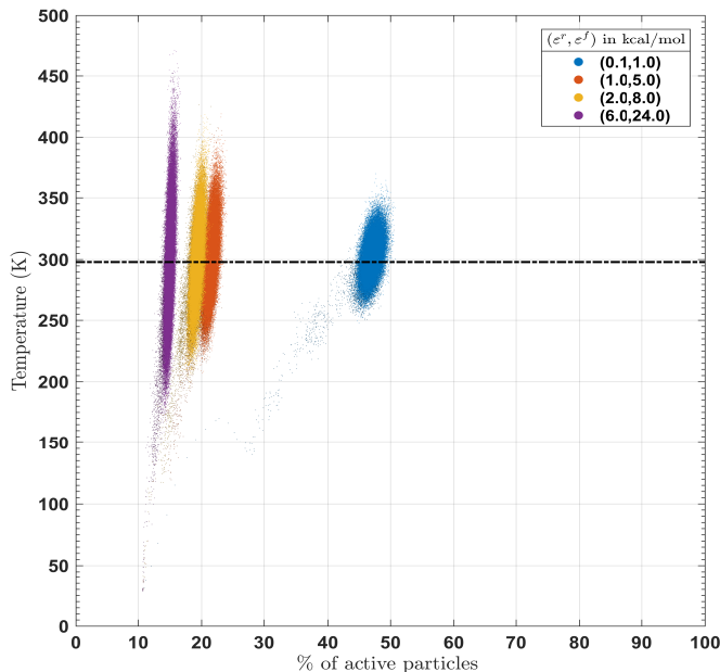
Figure 9: Temperature profile for NaCl + water mixture with an ionic concentration of 10.0 molal. Different restraining parameters (\epsilon^r, \epsilon^f) were tested on water molecules. Na and Cl are always active. Black line corresponds to the target temperature ( 298 K ).
