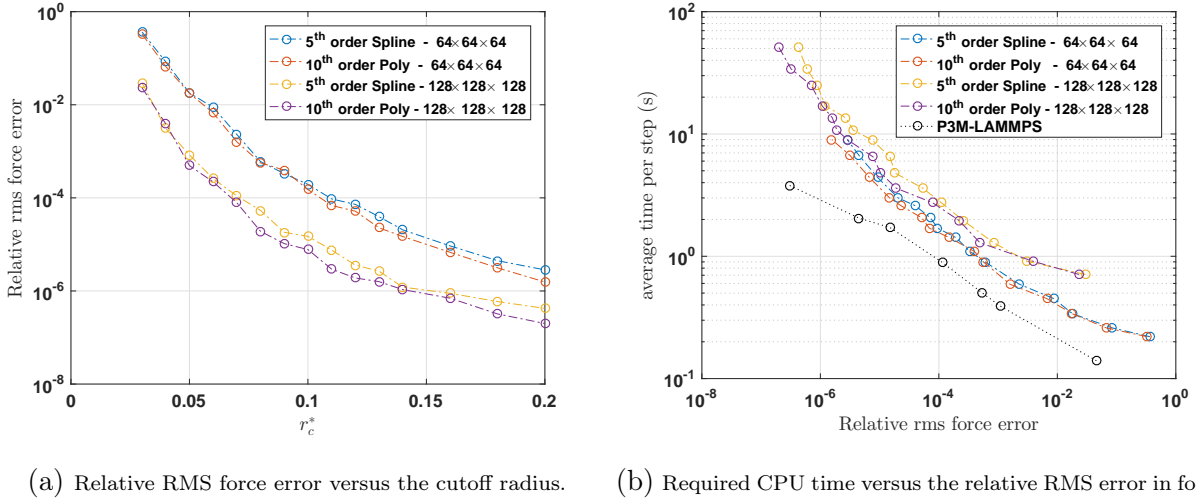
Figure 5: Evaluation of our implementation of MCM in LAMMPS on System A (64000 particles). The 10 th order polynomial function and the 5 th order B-spline were compared on 64^3 and 128^3 Grid. r_c^* = \frac{r_c}{L} is the normalized radius of the charge density.
