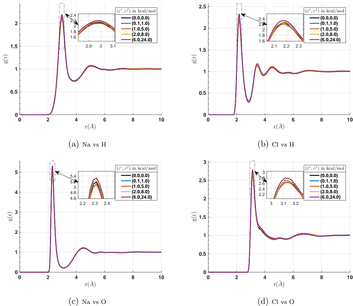
Figure 10: Ion-water pair distribution functions using ARMD with the NaCl/ \epsilon force field at 298 K the rigid water model SPC/ \epsilon and an ionic concentration of 10.0 molal. Different restraining parameters ( \epsilon^r, \epsilon^f ) were tested on water molecules. Na and Cl are always active. Black line corresponds to a standard molecular dynamics simulation of the system.
