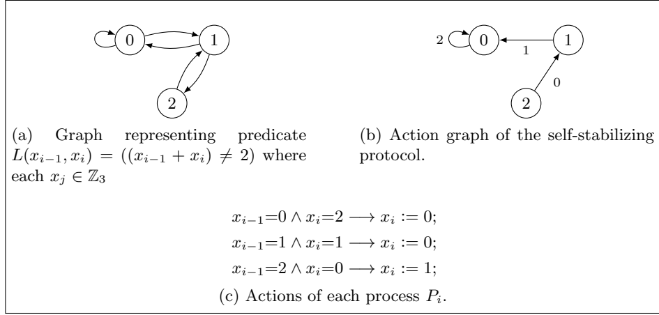
Fig. 3: Synthesis of parameterized Sum-Not-2.
