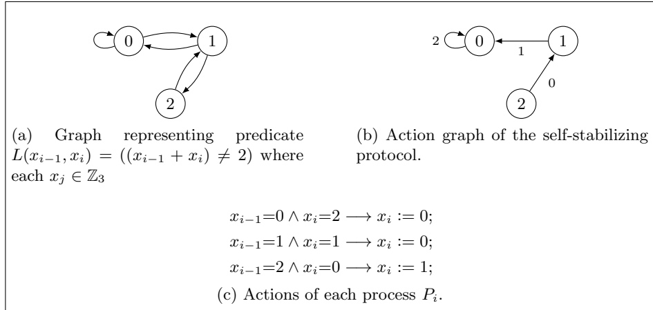
Fig. 3: Synthesis of parameterized Sum-Not-2.
