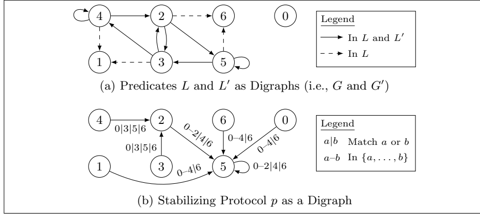
Fig. 2: Synthesis of stabilization to \forall i : L(x_{i-1}, x_i) , where L(x_{i-1}, x_i) \stackrel{\text{def}}{=} ((x_{i-1}^2 + x_i^3) \bmod 7 = 3) and x_i \in \mathbb{Z}_7 .
