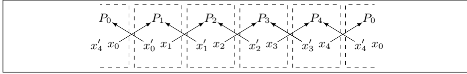
Fig. 5: Topology for bidirectional ring protocol p' in Theorem 8. Each process P_i owns x'_{i-1} and x_i .
