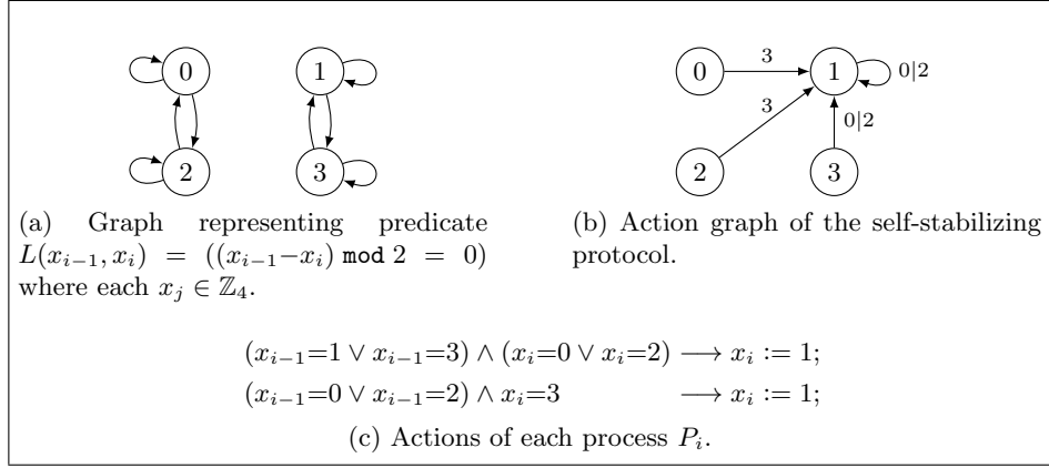
Fig. 4: Synthesis of parameterized Even Difference.
