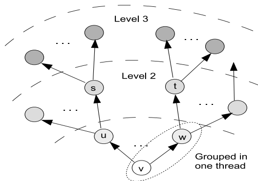
Fig. 1. Locality-Based Relaxation.
