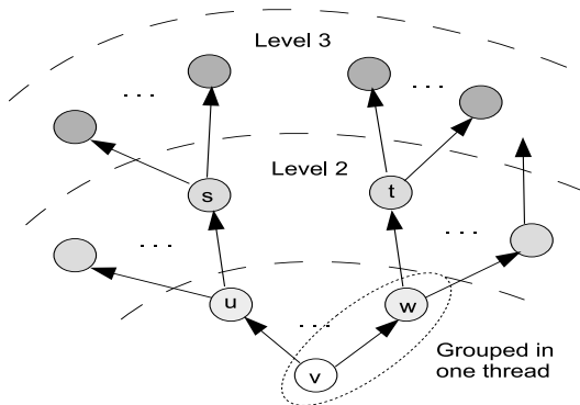
Fig. 1. Locality-Based Relaxation.
