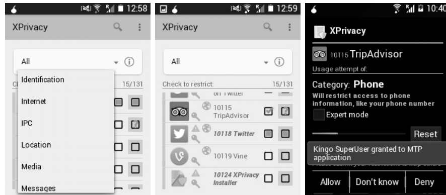
Figure 3. XPrivacy setup.
