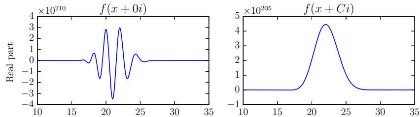
FIGURE 2. Real part of f(z) for z = x + 0i on the real line (left) and for z = x + Ci passing near the saddle point (right), here with parameters a = \frac{1}{2}, n = 500 , where integrating along the real line results in about five digits of cancellation.
