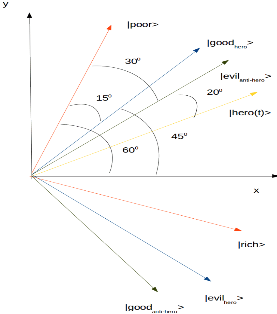
Fig. 1: Orientation between the bases M_{\text{hero}} , M_{\text{anti-hero}} and W on the xy plane. The unit vectors of the M_{\text{hero}} basis are in blue, the ones of the M_{\text{anti-hero}} are in black while the unit vectors of W are in red. Each one of these bases consists of orthonormal vectors.
