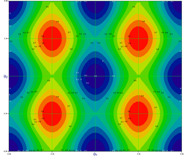
Figure 3. The levels of the function V(0, \theta) for the system (12)
