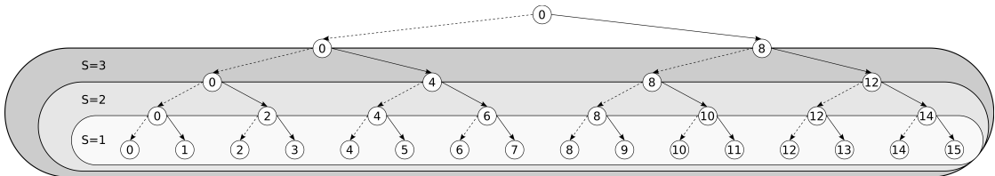
Figure 1: Communication tree for a broadcast collective with 16 MPI tasks. S is the number of steps (tree levels) running on application cores. Plain edges are communications. Vertices are the MPI tasks.
