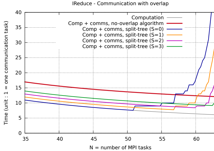
Figure 3: Model of communication/computation overlap for operations constant-size buffer (broadcast, reduce) on 64 cores.
