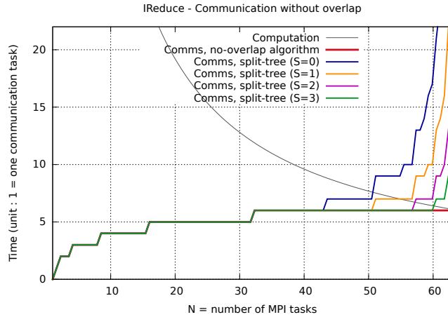
Figure 2: Model of communication cost for operations with constant-size buffer (broadcast, reduce) on 64 cores.
