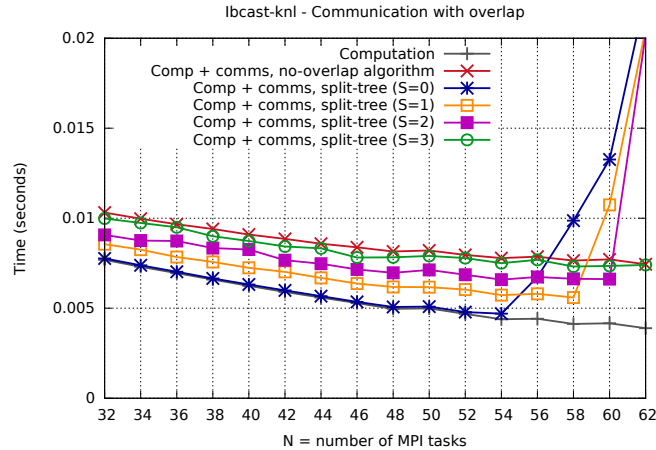
Figure 5: Result of split-tree algorithm with different values of S , for MPI_Ibcast with constant-size buffer of 2MB on 64 cores (KNL).
