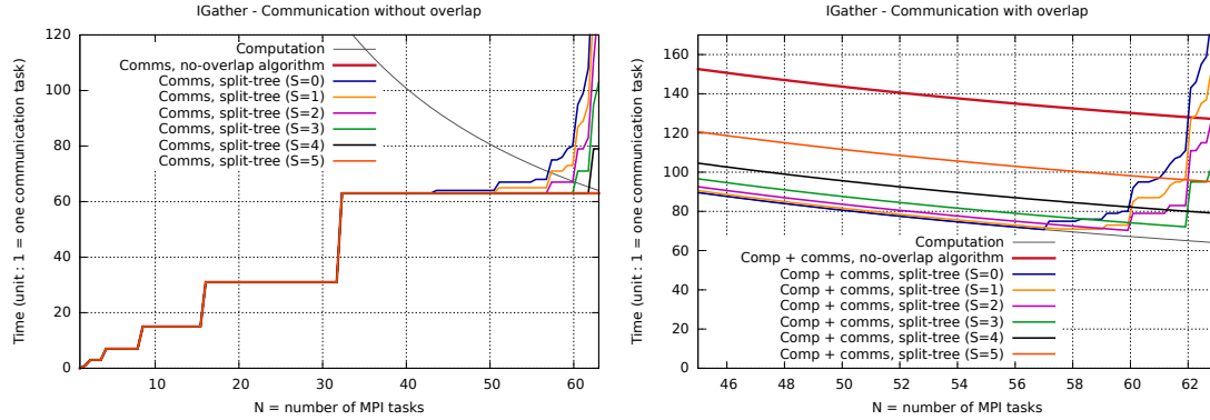
Figure 4: Model of communication cost (left) and communication/computation overlap (right) for operations with increasing buffer size (scatter, gather) on 64 cores.
