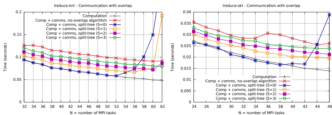
Figure 6: Result of split-tree algorithm with different values of S , for MPI_Ireduce with constant-size buffer of 2MB on KNL (left) and Skylake (right) processors.
