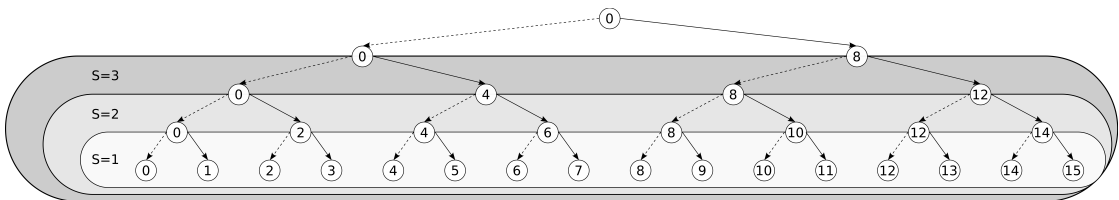
Figure 1: Communication tree for a broadcast collective with 16 MPI tasks. S is the number of steps (tree levels) running on application cores. Plain edges are communications. Vertices are the MPI tasks.
