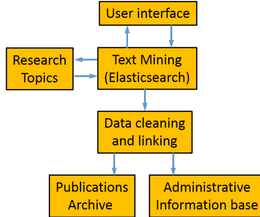
Figure 8: Components schema of LookinLabs.
