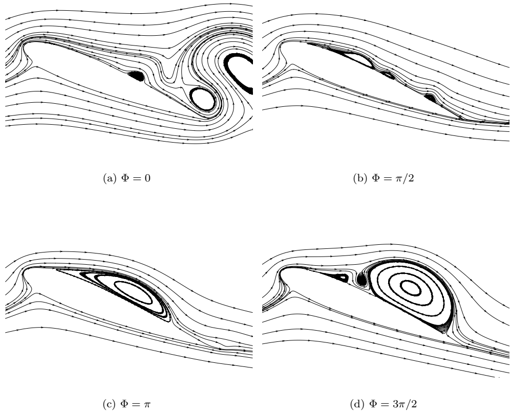
Figure 29: Streamlines with optimal parameters at 22^\circ
