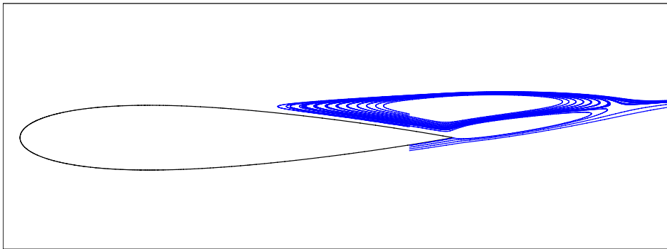
(c) NACA 0015
