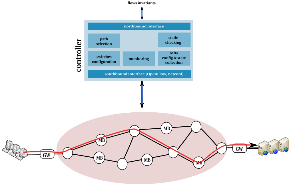
Fig. 2. Architecture components.
