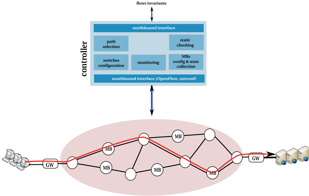
Fig. 2. Architecture components.
