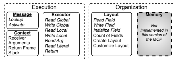
Fig. 2: Our Metaobject Protocol is designed to enable unforeseen software adaptations by providing access for inspecting and modifying the VM level. The operations highlighted in italics represent behavioral aspects, while the others represent structural aspects of the VM.
