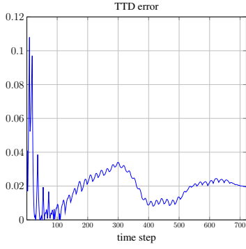
Fig. 5: Validation of the averaged model regarding total travel distance. The data plotted are computed as \frac{|\text{TTD}(\bar{t})^{\text{signalized}} - \text{TTD}(t)^{\text{averaged}}|}{\text{TTD}(t)^{\text{signalized}}}
