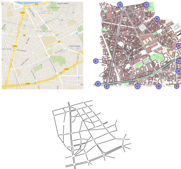
Fig. 10: From top left, clockwise: a map of Grenoble downtown; the corresponding Aimsun model used in the microscopic experiments, with markers for the detector positions that correspond to the inflows of the model (see also Figure 11); the directed graph describing this road network. A demo of our experiments is available online [39].
