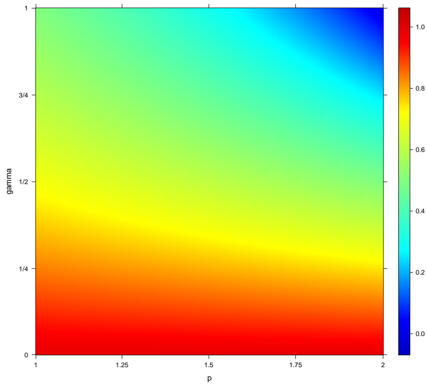
Figure 1: Behaviour of (p, \gamma) \mapsto \kappa(p, \gamma) for p \in [1, 2] and \gamma \in (0, 1) .
