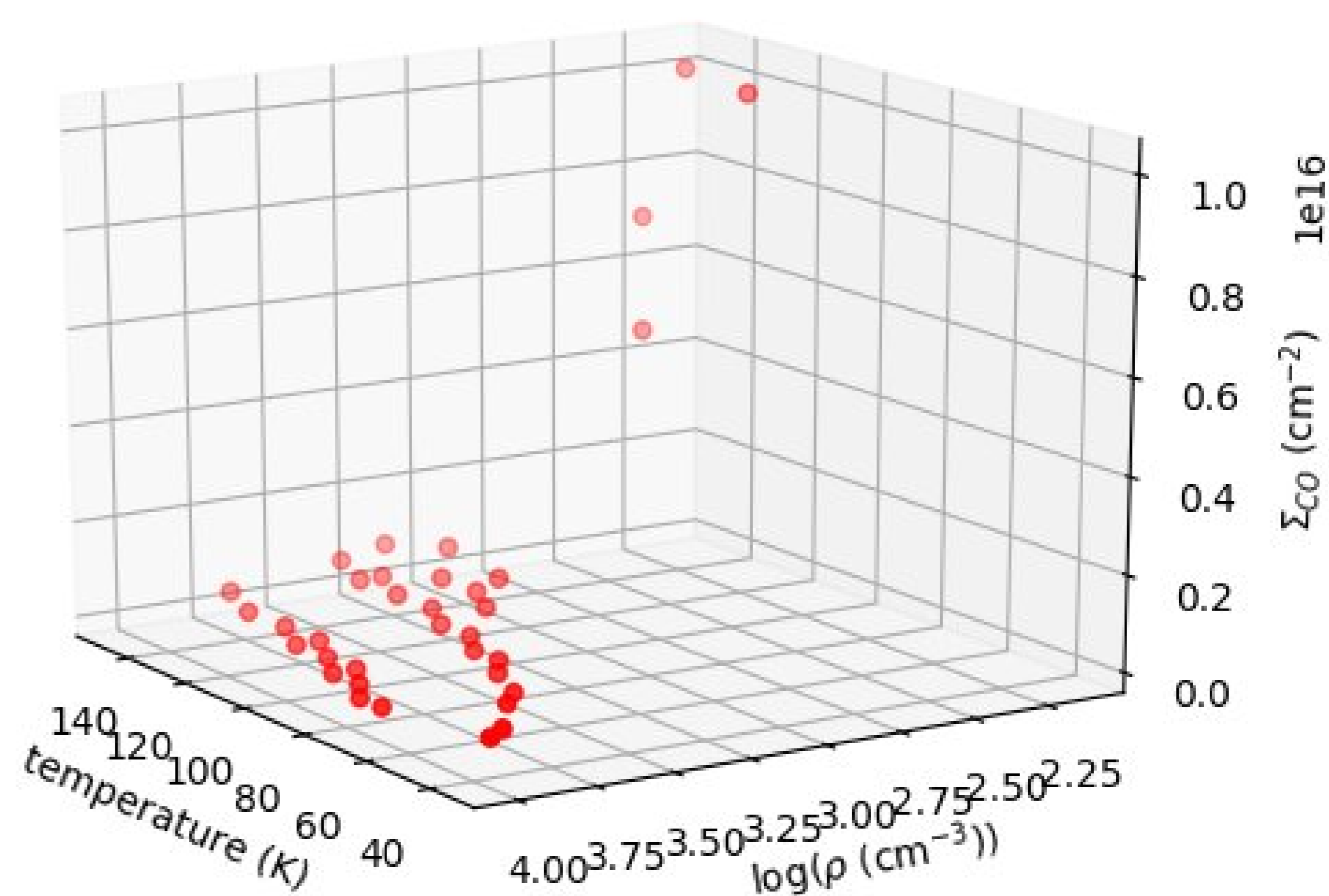
Fig 4) RADEX input that is consistent with both CO(3-2) and CO(4-3) emission of the excess component while keeping the ^{13}CO(2-1) and C^{18}O(2-1) emission sufficiently low.
