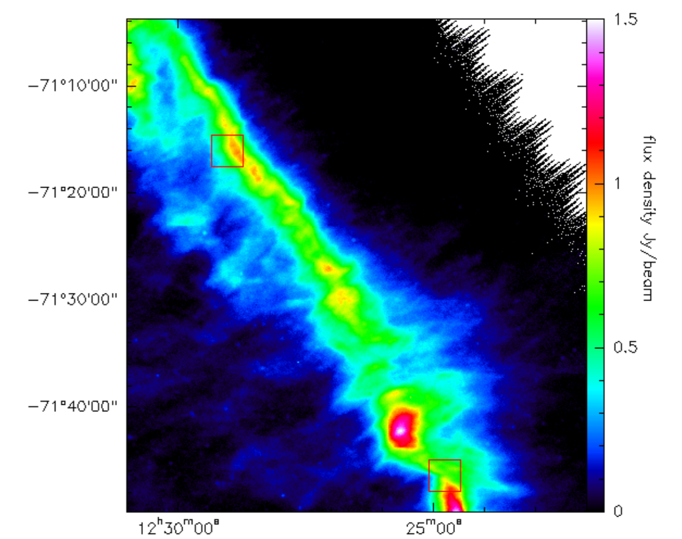
Fig 2 (above): A part of the Herschel 250\mu m map of Musca [7]. The two red boxes are the 2' \times 2' maps that were observed with APEX to look for indications of shocks.
