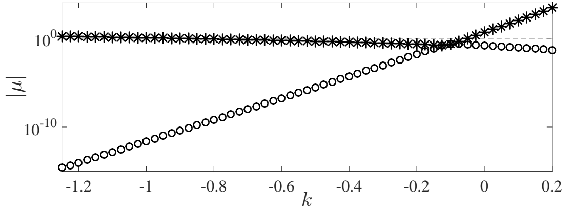
Figure 15: Magnitude of the Floquet multipliers for different values of k for the TUPO2 controlled by the aPBC.
