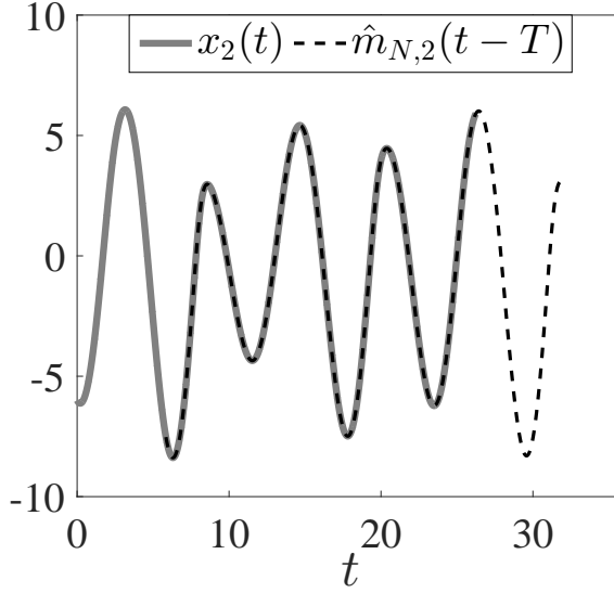
Figure 18: Current time and shifted future time trajectories of the Rössler system for k = 0 , k_o = 10 and N = 102 .
