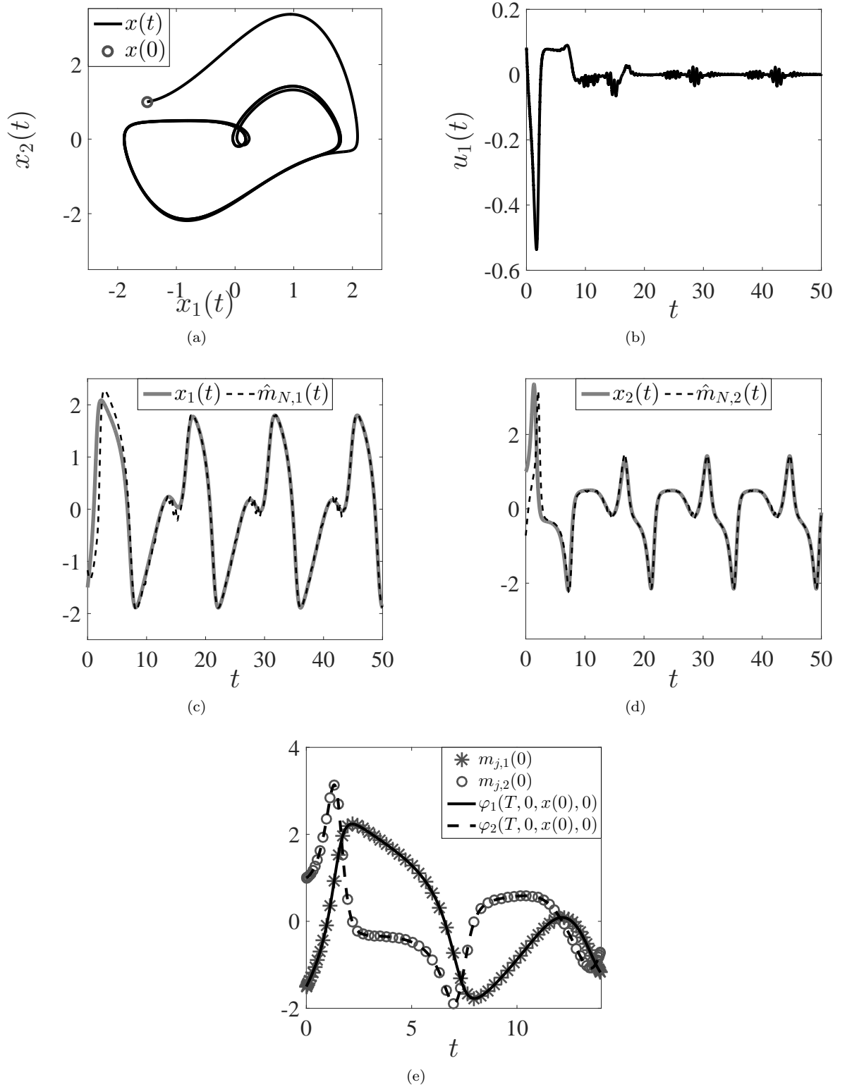
Figure 11: aPBC applied with N = 67 , k = 0.25 and k_o = 10 . (a) Trajectory in state space; (b) time-series of the control signal; (c) and (d) time-series of the actual and predicted state variables; (e) time-series of \varphi(T, 0, x(0), 0) and the initial value of the predicted states m_j(0) .
