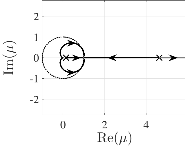
Figure 14: Root locus chart for the Floquet multipliers of the TUPO2 using the DFC. In black, the four largest magnitude Floquet multipliers for positive control gain k . In dark gray, the largest magnitude Floquet multiplier for negative control gain k . The Floquet multipliers of the free system orbit are represented by ( \times ) and the unit circle by dashed dark gray.
