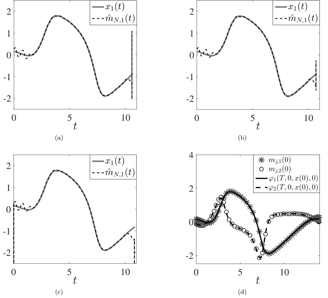
Figure 13: Time-series of a trajectory when applying the aPBC with N = 62 and: (a) k = 0 and k_o = 10 ; (b) k = 0.25 and k_o = 10 ; (c) k = 0.25 and k_o = 1000 ; (d) time-series of \varphi(T, 0, x(0), 0) and the initial value of the predicted states m_j(0) .
