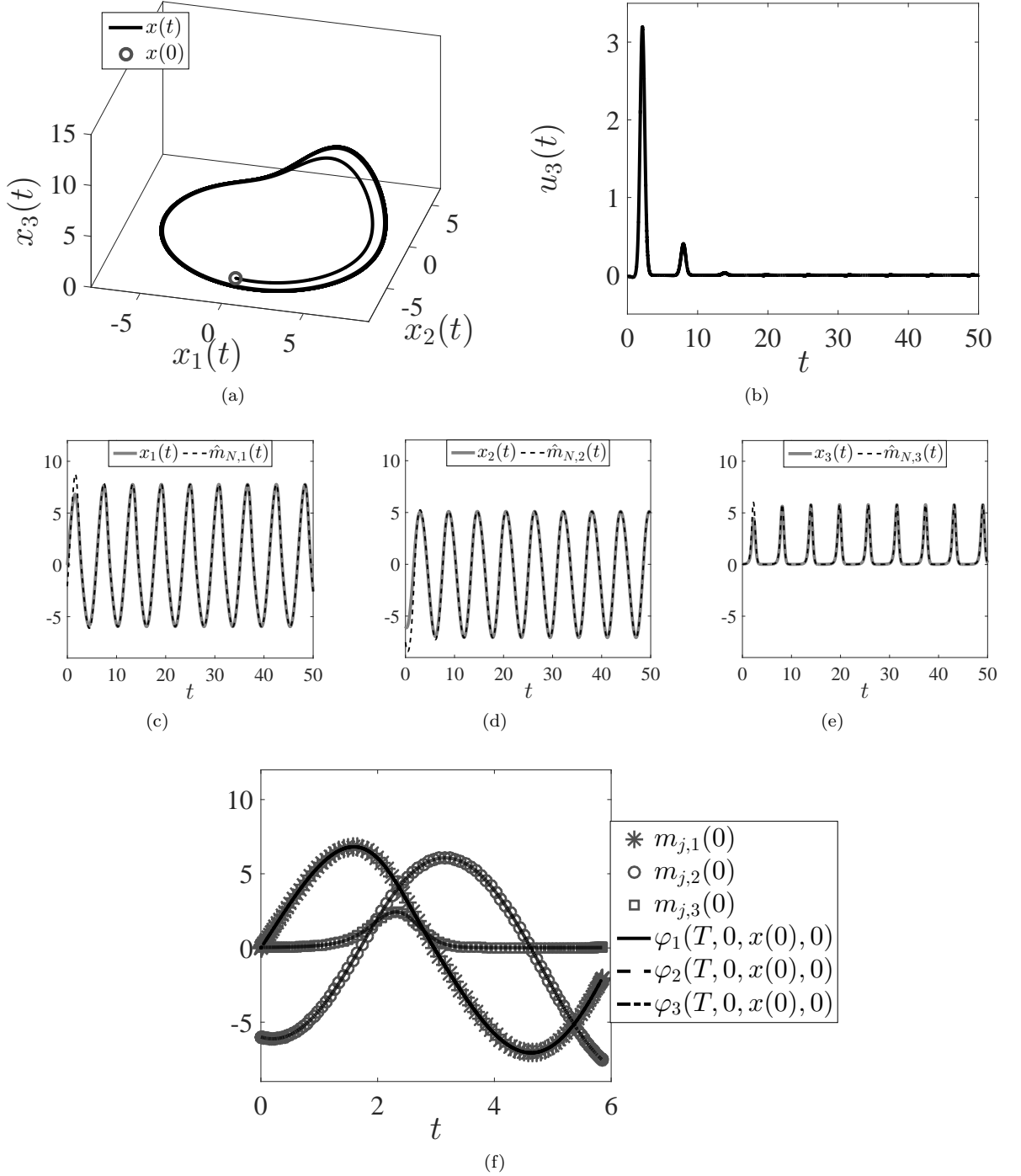
Figure 22: aPBC applied to the Rössler system with N = 102 , k = 1.85 and k_o = 10 . (a) Trajectory in state space; (b) time-series of the control signal; (c), (d) and (e) time-series of the actual and predicted state variables; (f) time-series of \varphi(T, 0, x(0), 0) and the initial value of the predicted states m_j(0) .
