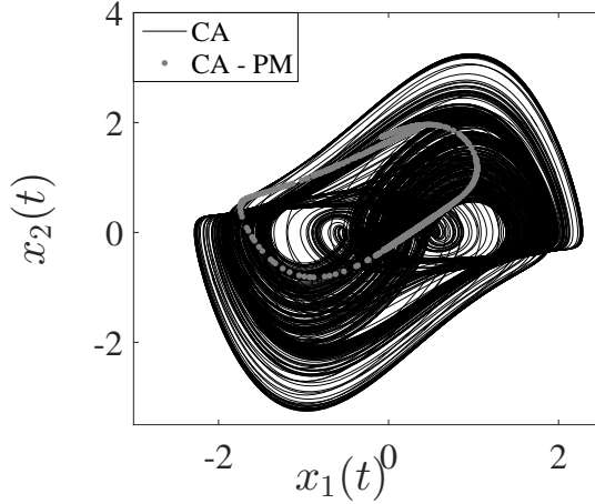
Figure 2: Forced van der Pol chaotic attractor in continuous-time (CA) and Poincaré map (CA - PM) for \omega = 0.45 , \eta = 1 and a = 0.988 .
