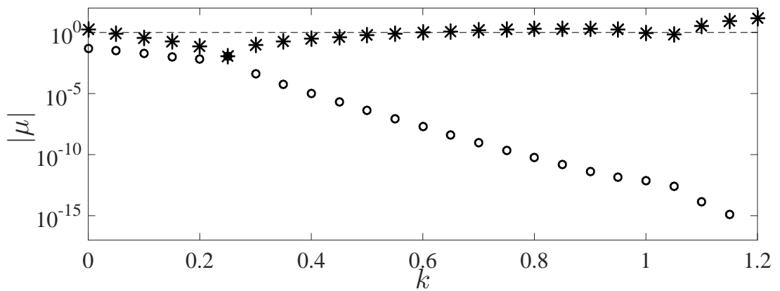
Figure 8: Magnitude of the two Floquet multipliers for different values of k for the TUPO1 controlled by the aPBC.
