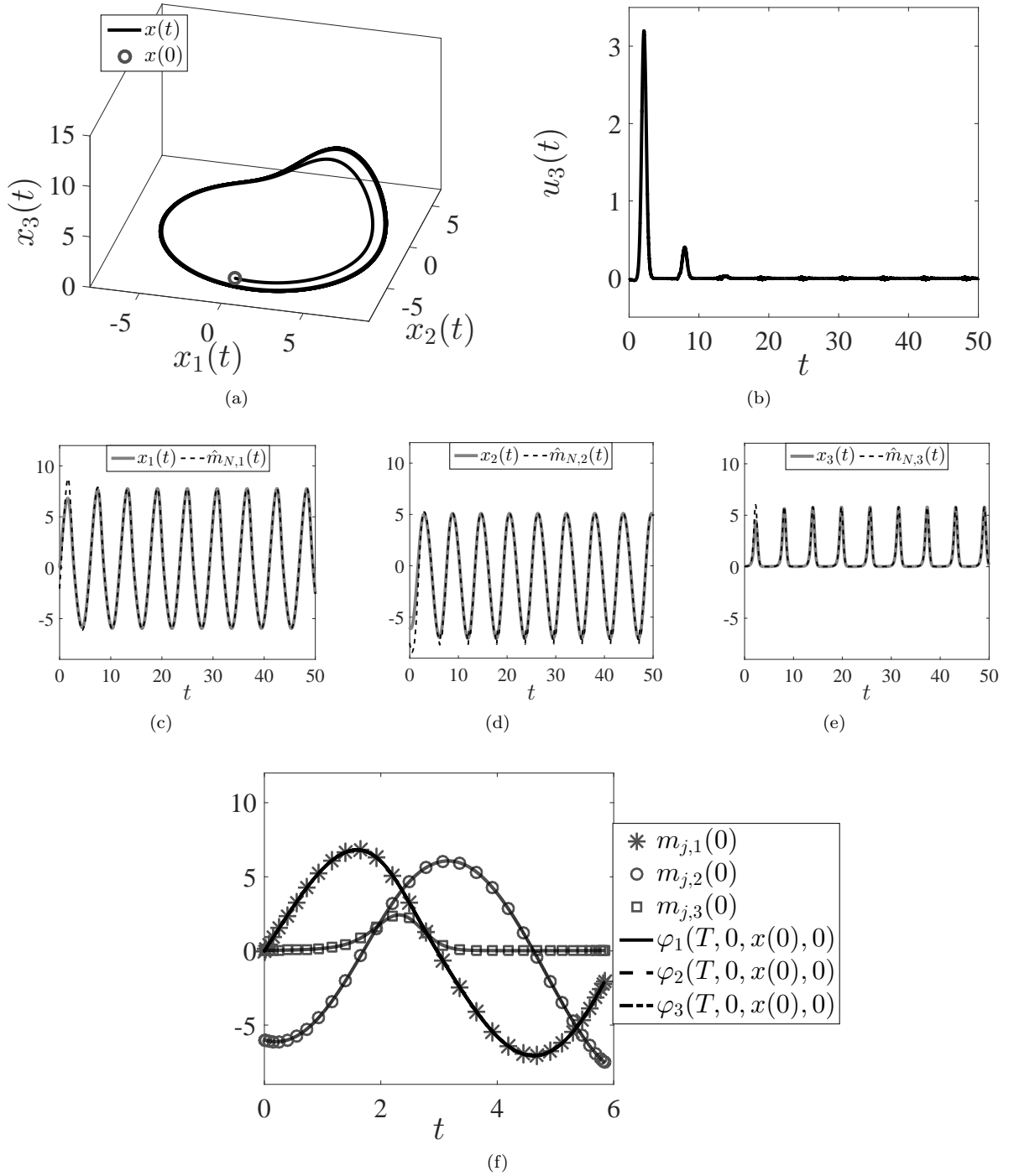
Figure 24: aPBC applied to the Rössler system with N = 32 , k = 1.85 and k_o = 10 . (a) Trajectory in state space; (b) time-series of the control signal; (c), (d) and (e) time-series of the actual and predicted state variables; (f) time-series of \varphi(T, 0, x(0), 0) and the initial value of the predicted states m_j(0) .
