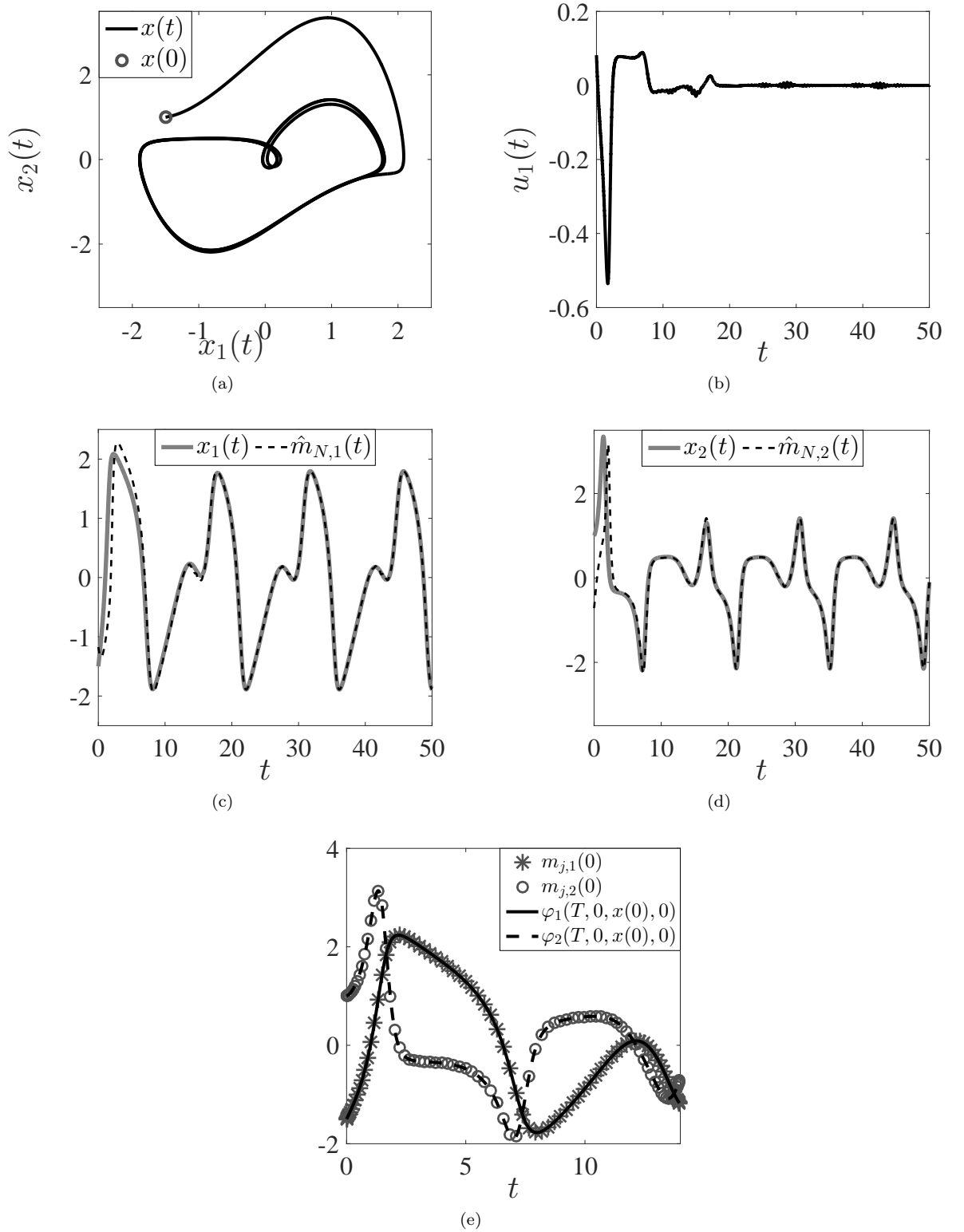
Figure 10: aPBC applied with N = 82 , k = 0.25 and k_o = 10 . (a) Trajectory in state space; (b) time-series of the control signal; (c) and (d) time-series of the actual and predicted state variables; (e) time-series of \varphi(T, 0, x(0), 0) and the initial value of the predicted states m_j(0) .
