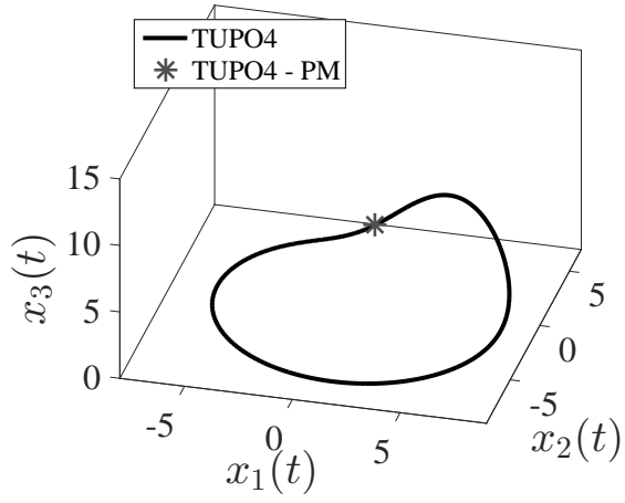
Figure 19: TUPO4 of Rössler system in continuous-time (line) and Poincaré map point (*) for \beta_1 = \beta_2 = 0.2 and \beta_3 = 4.5 .
