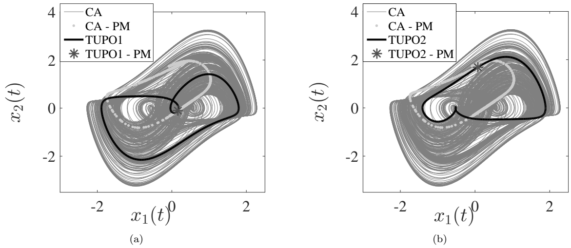
Figure 7: Target UPOs (TUPO1 and TUPO2) embedded in the chaotic attractor (CA) of the forced vdP oscillator. The points for the target UPOs and the chaotic attractor in the Poincaré map (PM) are represented by * and •, respectively.
