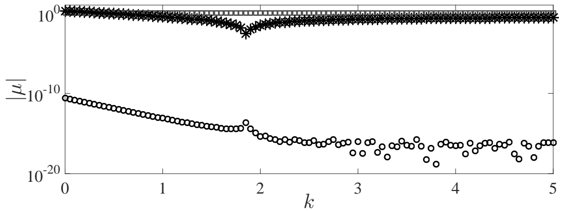
Figure 20: Magnitude of the Floquet multipliers for different values of k for the TUPO4 controlled by the aPBC.
