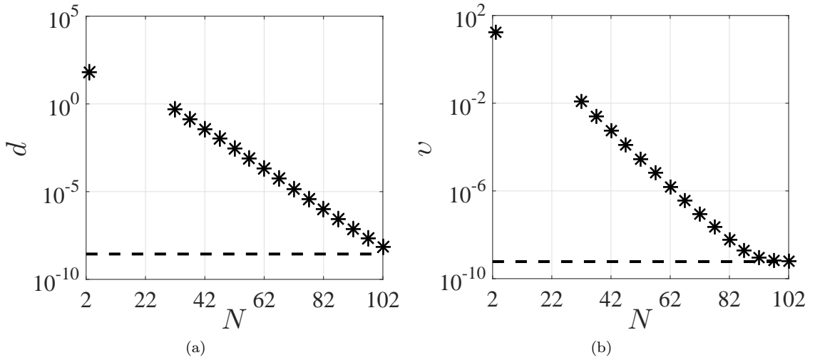
Figure 21: Indexes (a) d and (b) \nu when applying aPBC to TUPO4 for different N with k = 1.85 and k_o = 10 . The bottom dashed line are the values of (a) d and (b) \nu computed with N = 152 and k_o = 50 used as reference.
