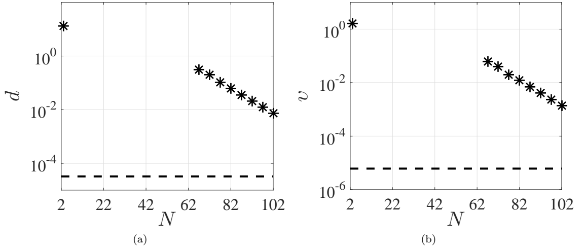
Figure 9: Indexes (a) d and (b) v when applying aPBC to TUPO1 for different N with k = 0.25 and k_o = 10 . Bottom dashed line are the values of (a) d and (b) v computed with N = 152 and k_o = 50 used as reference.
