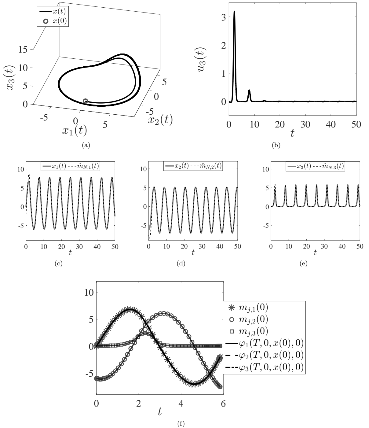
Figure 23: aPBC applied to the Rössler system with N = 52 , k = 1.85 and k_o = 10 . (a) Trajectory in state space; (b) time-series of the control signal; (c), (d) and (e) time-series of the actual and predicted state variables; (f) time-series of \varphi(T, 0, x(0), 0) and the initial value of the predicted states m_j(0) .
