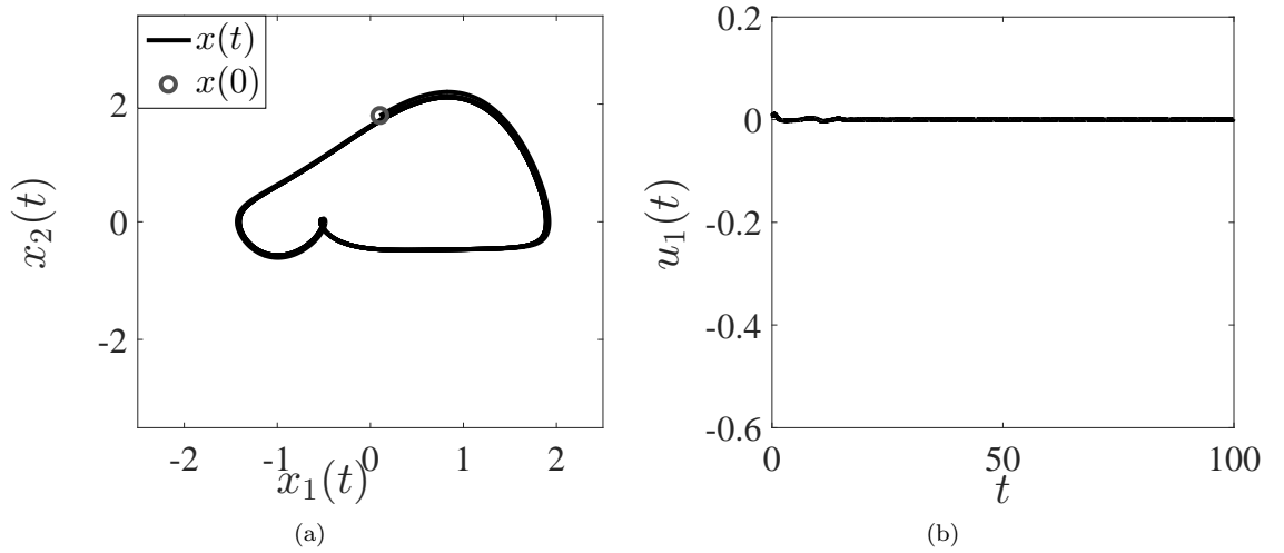
Figure 16: TUPO2 of forced vdP oscillator stabilized using aPBC with k = -0.125 and x(0) = [0.1 \ 1.8]^T . (a) State space trajectory and (b) time series of the control effort.
