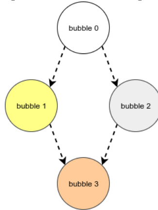
Figure 2.6: Bubble task-graph
