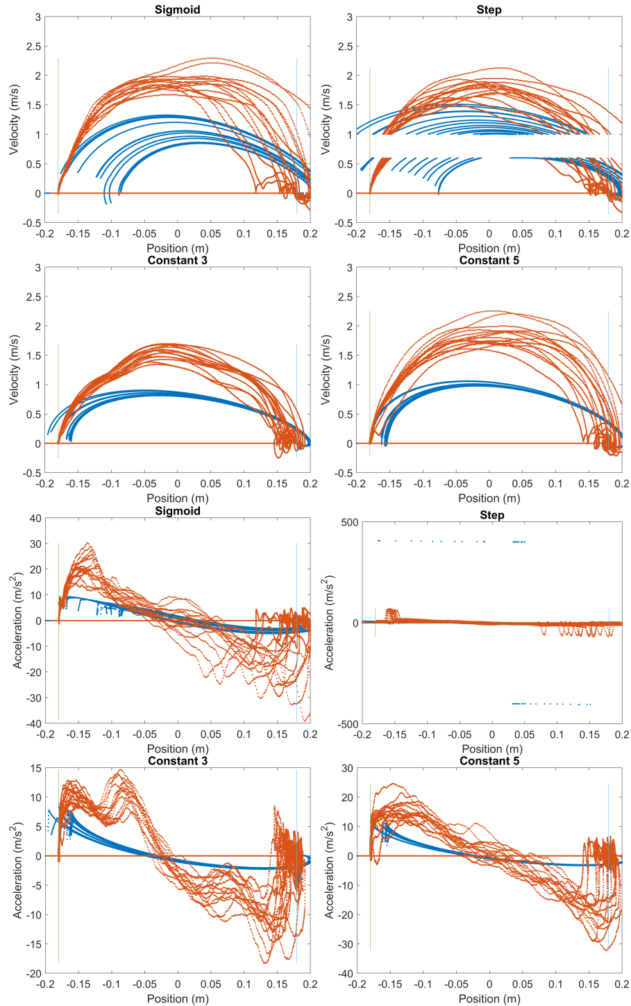
Fig. 10. Top: Phase space plot of pointer velocity predicted by the models (blue), as well as phase space plot of the actual pointer (red) for one user. For the Step TF, there is a jump in velocity when the velocity crosses the step both during acceleration and deceleration. This phenomenon is replicated by the model (blue). Bottom: Hooke plots of pointer acceleration predicted by the model (blue), as well as the actual pointer acceleration (red). The reached acceleration is higher than for constant gain. The Step TF results in steep acceleration and deceleration spikes when the velocity crosses the step. This behavior is replicated by the model. For constant gain 3, this user shows two acceleration spikes per movement. One hypothesis might be that this user starts to accelerate the mouse, but only overcomes the static friction of the arm on the table slightly later, resulting in a second acceleration spike.
