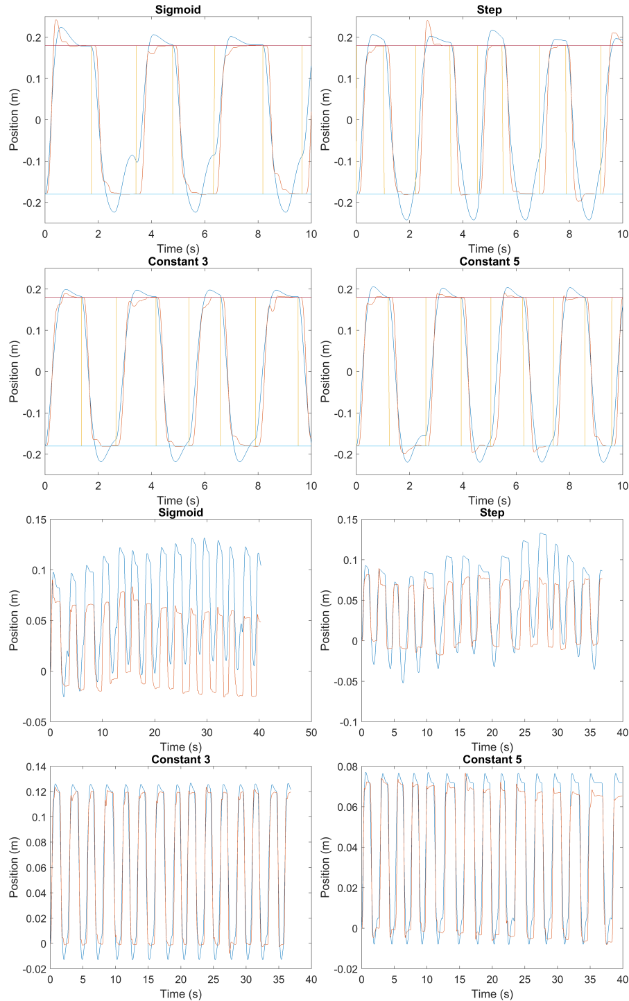
Fig. 9. Top: Time Series of pointer position predicted by the model (blue), as well as the actual pointer position (red) for one user. The target position is shown for orientation (yellow). Bounds of the targets are shown as horizontal colored lines (ID 8). The model can predict the position over time of the pointer rather well. However, no apparent differences in the dynamic behavior with the four transfer functions are visible in the time series. Bottom: Time Series of mouse position predicted by the four models (blue), as well as the actual mouse position (red) for one user. It can be seen that the mouse of the user (red) is drifting considerably when using a PA function, but less so with a constant gain. The reason for this is that users reach different velocities when moving left vs. right. Because the PA function increases the gain as a function of velocity, the mouse is drifting into the direction where higher velocities are reached. This effect is stronger for the sigmoid PA function than for the step PA function.
