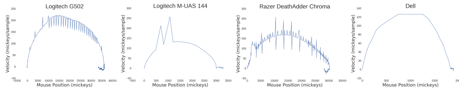
Fig. 2. Noise for different mice. Logitech G502, Logitech UAS144, Razer DeathAdder, and a Dell mouse, respectively. The noise gets amplified by PA functions. The Dell mouse seems to exhibit less noise but provides much lower temporal and spatial resolution.
