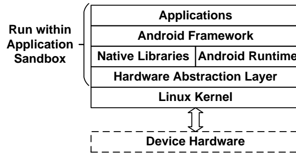
Figure 1. Android security architecture [1].
