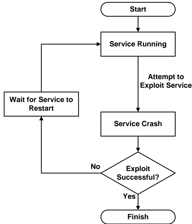
Figure 4. Brute-force execution.
