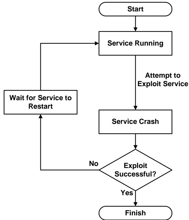
Figure 4. Brute-force execution.
