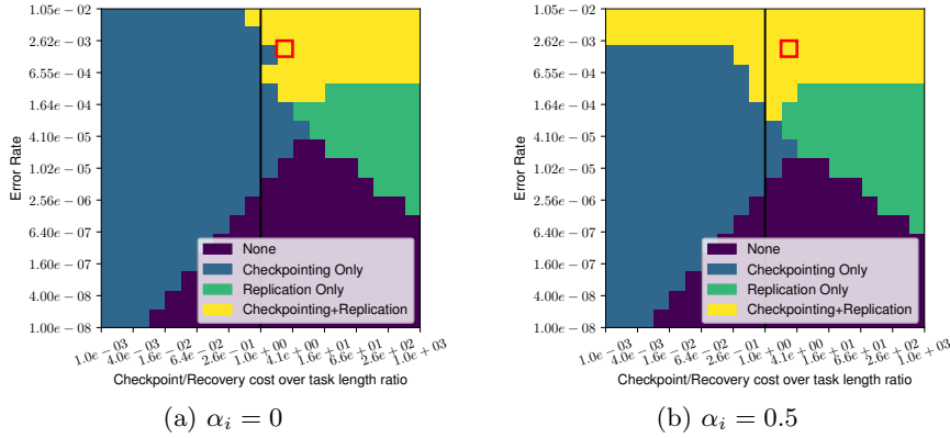
Figure 1: Impact of checkpoint/recovery cost and error rate on the usage of checkpointing and replication. Total work is fixed to 10,000s and is distributed uniformly among n = 20 tasks (i.e., T_1 = T_2 = \dots = T_{20} = 500 s).
