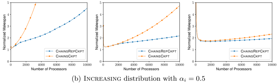
Figure 20: Comparison of the CHAINSCKPT and CHAINSREPCKPT strategies for different numbers of processors, with different model parameter values for the checkpointing cost (a_i, b_i, c_i) of (100, 10000, 1) (left), (100, 100000, 0.1) (middle) and (100, 1000000, 0.01) (right).
