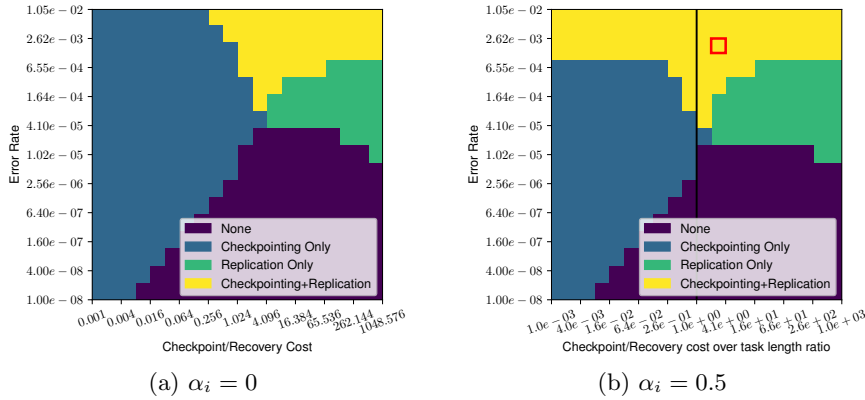
Figure 8: Impact of checkpoint/recovery cost and error rate on the usage of checkpointing and replication. Total work is fixed to 10,000s, there are n = 20 tasks and the work is distributed according to the INCREASING distribution.
