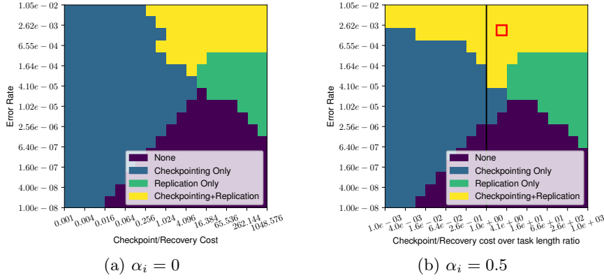
Figure 11: Impact of checkpoint/recovery cost and error rate on the usage of checkpointing and replication. Total work is fixed to 10,000s, there are n = 20 tasks and the work is distributed according to the RANDOM distribution.
