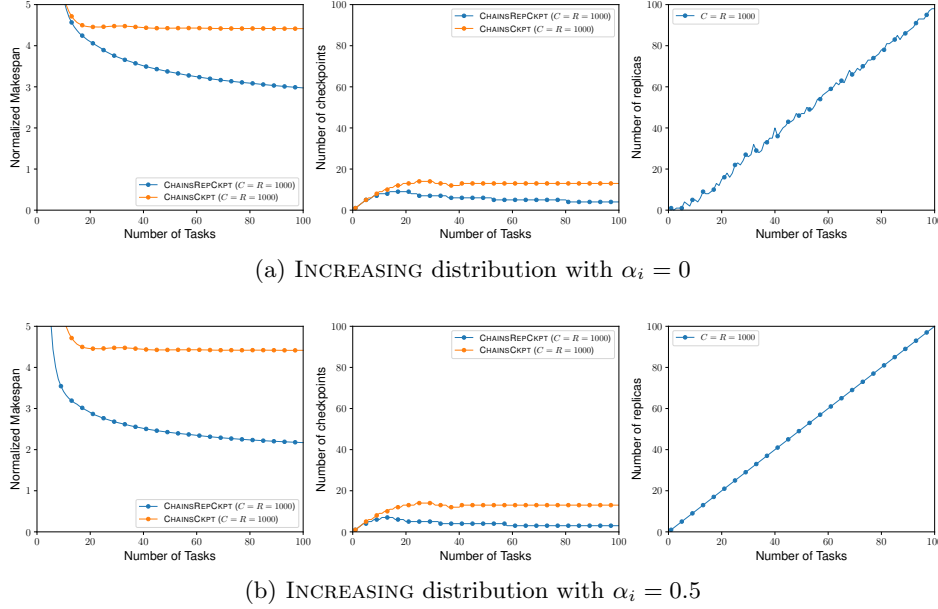
Figure 12: Comparison of the CHAINSCkPT and CHAINSREPCkPT strategies for different numbers of tasks: impact on the makespan (left), number of checkpoints (middle) and number of replicas (right) with an error rate of \lambda_{indp} = 10^{-3} and a constant checkpointing/recovery cost C_i^{morep} = C_i^{rep} = 1000s .
