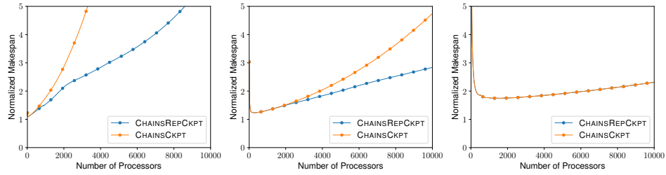
(a) RANDOM distribution with \alpha_i = 0
