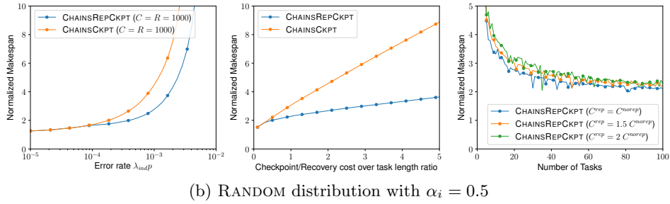
Figure 19: Impact of error rate \lambda_{indP} (left), checkpoint cost (middle) and ratio \alpha between the checkpointing cost for replicated task C_i^{rep} over non-replicated tasks C_i^{norep} (right).
