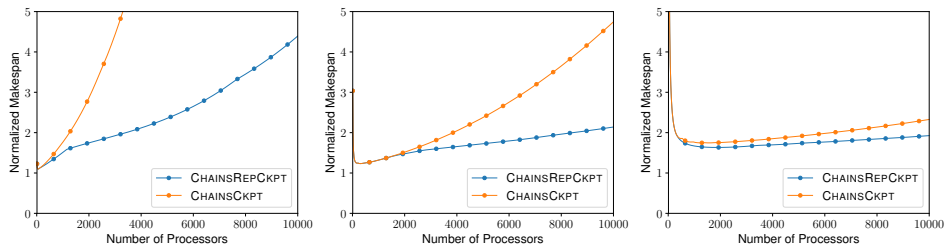
(b) DECREASING distribution with \alpha_i = 0.5
