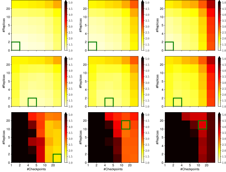
Figure 7: Impact of the number of checkpoints and replicas on the normalized expected makespan for \lambda = 10^{-4} (top), \lambda = 10^{-3} (middle) and \lambda = 10^{-2} (bottom) and for checkpointing costs equal to 0.5 \times T_i^{norep} (left), 1 \times T_i^{norep} (middle) and 2 \times T_i^{norep} (right), with C_i^{norep} = C_i^{rep} under UNIFORM work distribution. The optimal solution obtained with CHAINSREPCKPT always matches the minimum simulation value and is highlighted in green.
