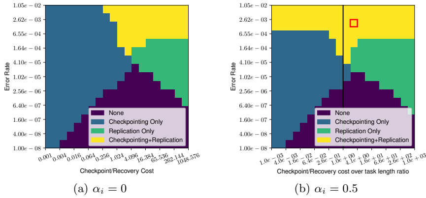
Figure 9: Impact of checkpoint/recovery cost and error rate on the usage of checkpointing and replication. Total work is fixed to 10,000s, there are n = 20 tasks and the work is distributed according to the DECREASING distribution.
