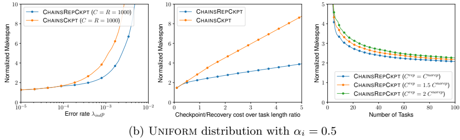
Figure 5: Impact of error rate \lambda_{indp} (left), checkpoint cost (middle) and ratio \alpha between the checkpointing cost for replicated task C_i^{rep} over non-replicated tasks C_i^{norep} (right).
