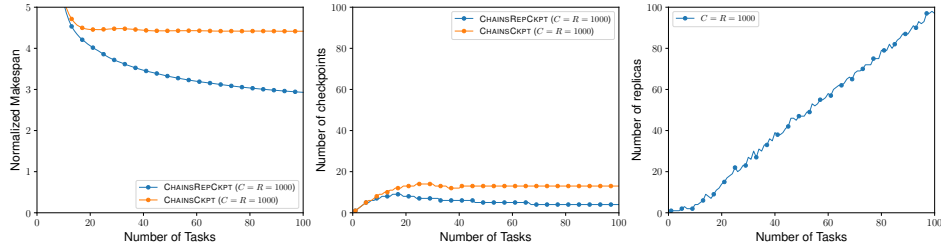
(a) DECREASING distribution with \alpha_i = 0
