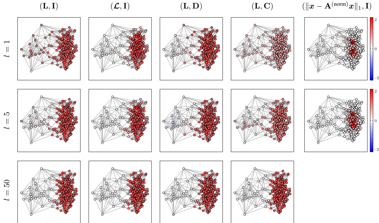
Fig. 6. Output of the ideal low pass filter \mathbf{H}_l applied to the normalized indicator function \mathbf{h}_{\text{blue}}^{(\mathbf{Q})} . \mathbf{H}_l keeps only the first l+1 spectral components (i.e., up to the graph frequency \lambda_l ). Note that \mathbf{H}_l depends on the (\Delta, \mathbf{Q}) -GFT.
