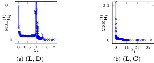
Fig. 4. I-MSE of the ideal low-pass filter \mathbf{H}_I applied to the normalized indicator function \mathbf{h}_{\text{blue}}^{(\mathbf{Q})} corresponding to (a) Fig. 3(d) and (b) to Fig. 3(e).
