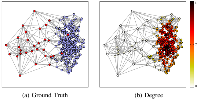
Fig. 2. Two cluster dataset input with a sparse cluster (left) and a dense cluster (right). (a) Ground truth clusters. (b) Vertex degrees from the 10-nearest neighbor graph Gaussian weights.
