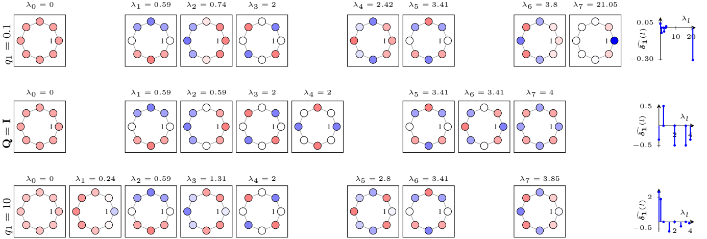
Fig. 1. (\mathbf{L}, \mathbf{Q}) -graph Fourier modes of the ring graph with N = 8 vertices. \mathbf{Q} = \text{diag}(q_1, 1, \dots, 1) with one choice of q_1 per row of the table, for increasing values of q_1 . Modes are not aligned on their index, but when they correspond either exactly (3 rd , 5 th , and 8 th column), or approximately, to highlight the impact of q_1 on the graph Fourier modes. Colors scale from deep blue for -1 to deep red for 1 and color being lighter as values get closer to 0 until white for 0 . Note that [\mathbf{u}_7]_1 = -3.08 for q_1 = 0.1 is out of this range. The last column shows the graph Fourier transform \widehat{\delta}_1 of the impulse \delta_1 .
