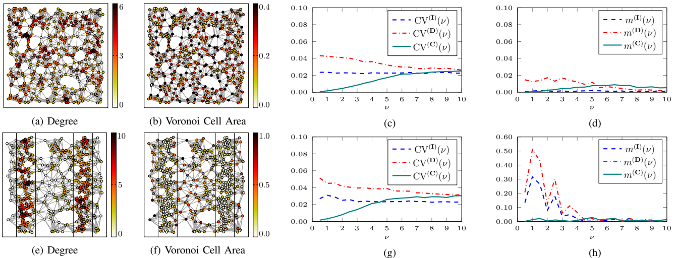
Fig. 3. Study of the graph energy of single cosine continuous signal \tilde{s}_\nu(x, y; \varphi) = \cos(2\pi\nu x_i + \varphi) sampled uniformly (a)-(d) and non-uniformly (e)-(h) as s_\nu(i; \varphi) = s_\nu(x_i, y_i; \varphi) . Example sampling with 500 samples (vertices) showing vertex degree ((a) and (e)), and Voronoi cell area ((b) and (f)) with colors. (c)-(d) and (g)-(h) 1000 samples (vertices), with results averaged over 500 sampling (graph) realizations. (c) and (g) coefficient of variation CV^{(\mathbf{Q})}(\nu) of the signal energy depending on the continuous frequency \nu . (d) and (h) maximum absolute deviation m^{(\mathbf{Q})}(\nu) of the normalized mean signal energy depending on the continuous frequency \nu .
