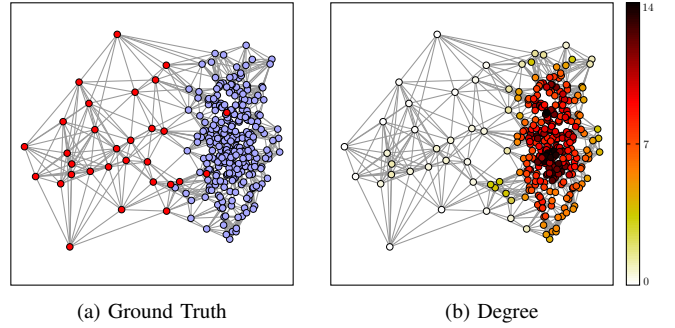
Fig. 1. Two cluster dataset input with a sparse cluster (left) and a dense cluster (right). (a) Ground truth clusters. (b) Vertex degrees from the 10-nearest neighbor graph Gaussian weights.
