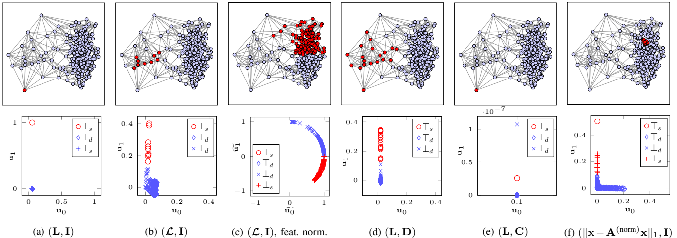
Fig. 2. Several spectral clustering results on the graph of Fig. 1. The smallest cluster is in dark red, and the largest cluster is in light blue. The second row of plots shows the input in the feature space, i.e. , to each vertex i is associated a point [[\mathbf{u}_0]_i, [\mathbf{u}_1]_i]^T in the spectral feature space. The set T_s (resp. T_d ) corresponds to the vertices in the sparse (resp. dense) cluster and correctly clustered. The set \perp_s (resp. \perp_d ) corresponds to vertices incorrectly clustered in the sparse (resp. dense) cluster. Colors in both rows of figures match for consistency. Fig. 2(a): (\mathbf{L}, \mathbf{I}) , Fig. 2(b) (\mathcal{L}, \mathbf{I}) with normalized feature vectors, Fig. 2(d) (\mathbf{L}, \mathbf{D}) , Fig. 2(e) (\mathbf{L}, \mathbf{C}) , and Fig. 2(f) (\Delta, \mathbf{I}) with \Delta(\mathbf{x}) = \|\mathbf{x} - \mathbf{A}^{(\text{norm})}\mathbf{x}\|_1 .
