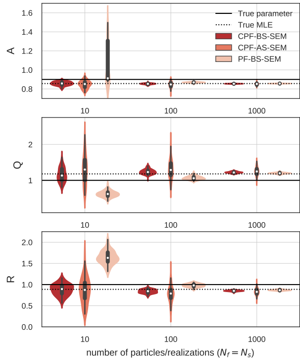
Figure 8. Comparison of the estimates of \theta = (A, Q, R) at iteration 100 of CPF-BS-SEM, CPF-AS-SEM, and PF-BS-SEM for the linear Gaussian SSM model (19) with true parameter \theta^* = (0.9, 1, 1) and T = 100 . These algorithms are run with different number of particles/trajectories ( N_f = N_s \in \{10, 100, 1000\} ). The true MLE (dotted line) is computed using KS-EM with 10^4 iterations.
