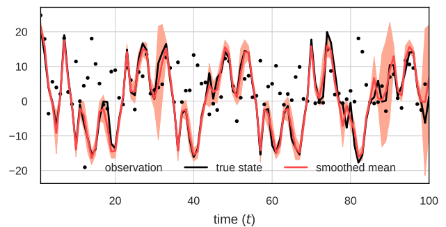
Figure 12. Reconstruction of the true state using CPF-BS-SEM with 10 particles/realizations on the Kitagawa model (20) given T = 100 observations. Smoothed means and 95% confidence intervals of all realizations simulated from last 10 iterations of the algorithm are presented.
