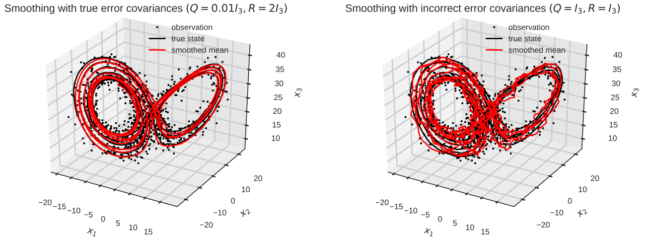
Figure 1. Impact of parameter values on smoothing distributions for the Lorenz-63 model. The true state (black curve) and observations (black points) have been simulated with \theta = (Q, R) = (0.01I_3, 2I_3) . The mean of the smoothing distributions (read curve) are computed using a standard particle smoother (Douc et al. 2009) with 100 particles. Results obtained with the true parameter values \theta^* = (0.01I_3, 2I_3) (left panel) and wrong parameter values \hat{\theta} = (I_3, I_3) (right panel).
