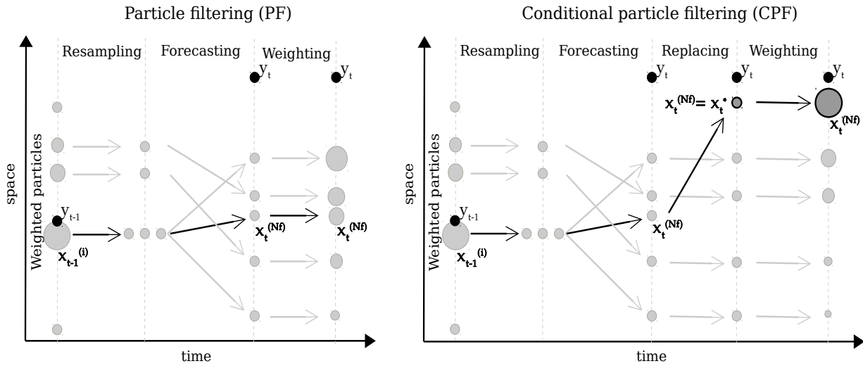
Figure 2. Comparison of PF and CPF schemes using N_f = 5 particles (light gray points) in time window [t - 1, t] on the SSM (1). The observation model is the identity function. The main difference is shown on black quivers as CPF replaces the particle x_t^{(N_f)} with conditioning particle x_t^* (dark gray point).
