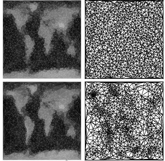
Figure 10: Top=level 21 reconstruction, 2326 triangles (left=data set, right=triangulation), Bottom=threshold reconstruction, 2388 triangles (left=data set, right=triangulation).
