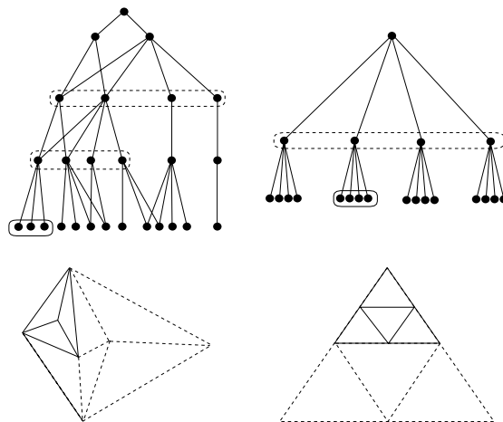
Figure 7: Including a wavelet coefficient: triangles lying outside the wavelet support are required.
