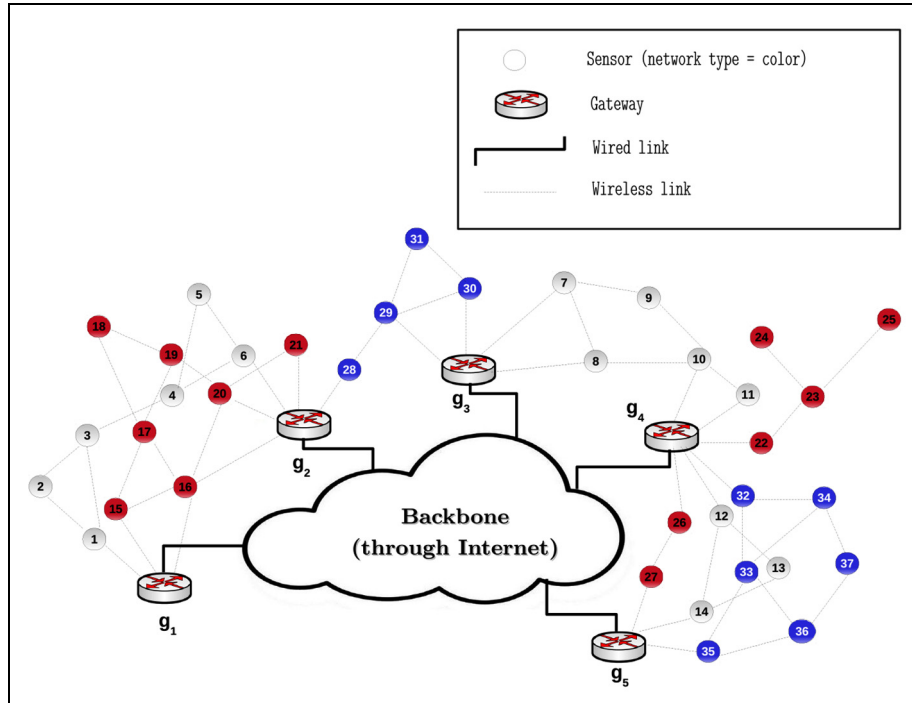
Figure 1. Backbone architecture for WSN interconnection.
