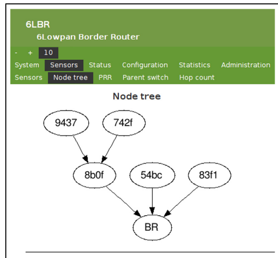
Figure 7. Home automation scenario: first gateway—stage 1.
