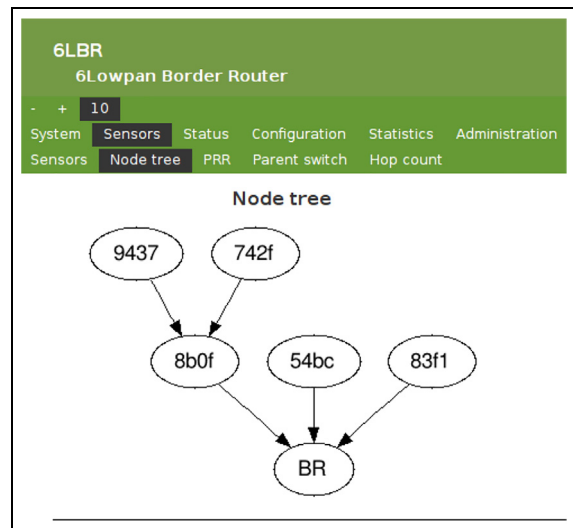
Figure 7. Home automation scenario: first gateway—stage I.
