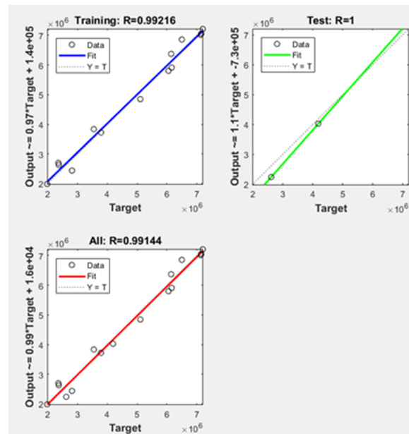
Fig. 3: Regression and Correlation. MatLab©R2016b
