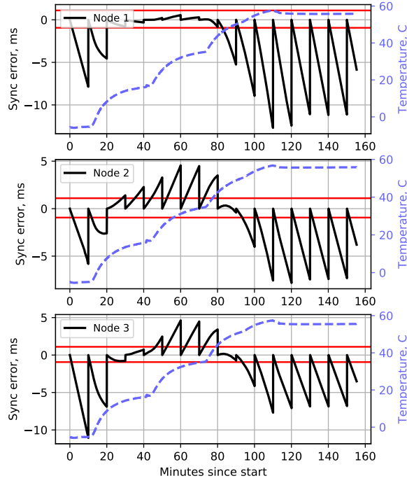
(a) Baseline TSCH, no compensation. |err|_{max} = 12.7 ms, |err|_{mean} = 2.58 ms
