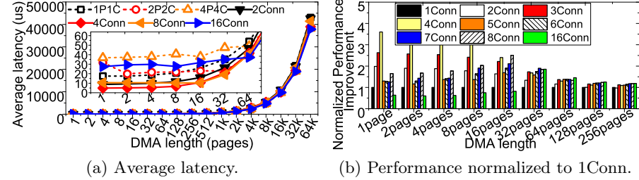
Fig. 3: Performance improvements of RMA with connection channels.
