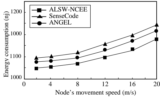
Fig. 4. Energy consumption with Node's movement speed (m/s).
