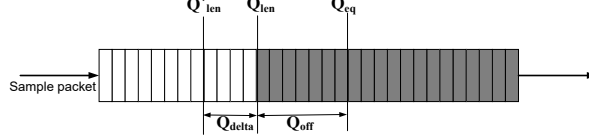
Fig. 4. Congestion detection in both input queue and output queue
