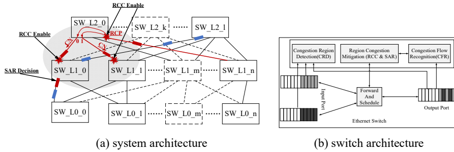
Fig. 3. Architecture of Regional congestion mitigation
