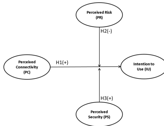
Figure 1. Research Model
