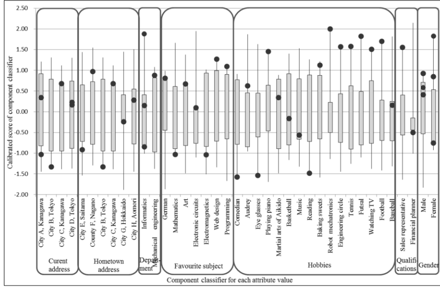
Fig. 2. Score distribution of component classifiers with bag-of-words and Random Forest
