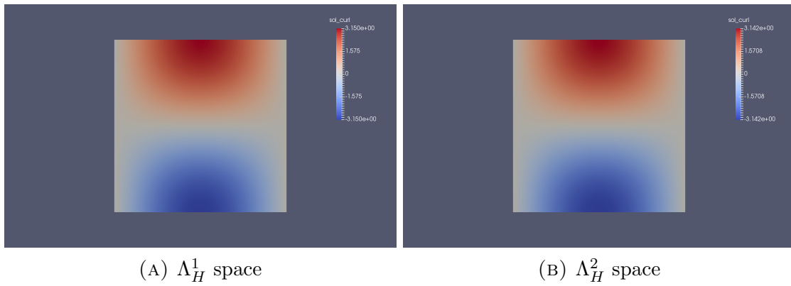
FIGURE 8. \text{curl } u_H on a 16 \times 16 mesh
