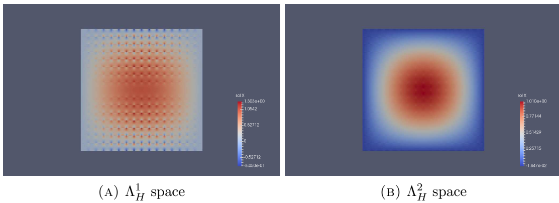
FIGURE 7. x_1 component of u_H on a 16 \times 16 mesh
