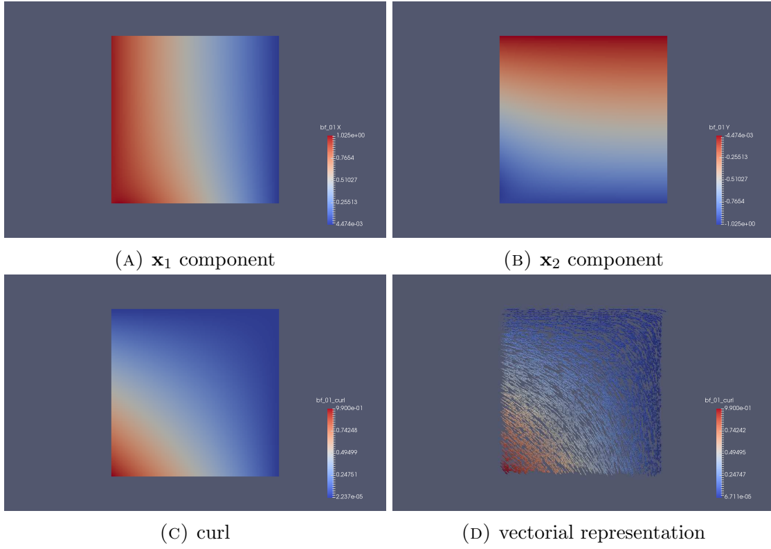
FIGURE 1. \hat{\mathbf{T}}\lambda^1
