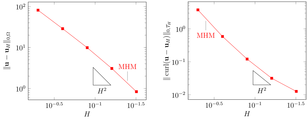
FIGURE 6. Convergence curves for second-order elements
