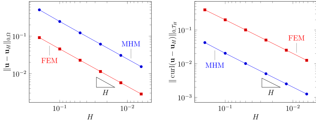
FIGURE 5. Convergence curves for first-order elements
