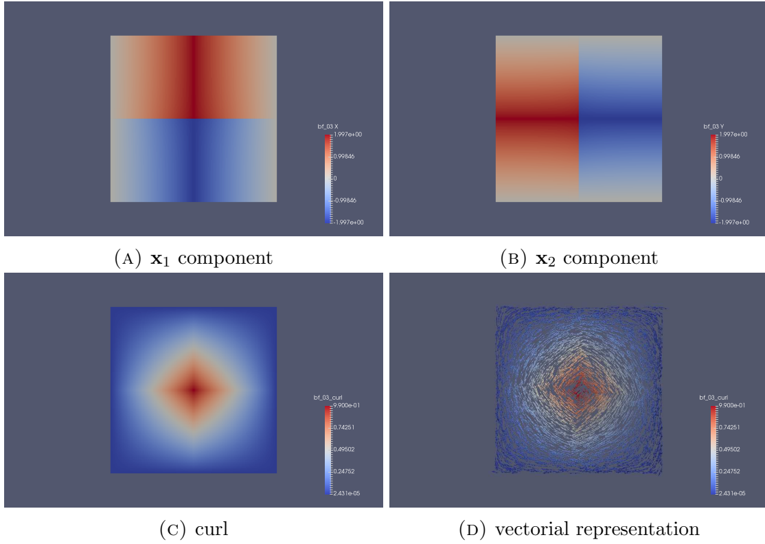
FIGURE 3. Nodal shape function T\psi^3
