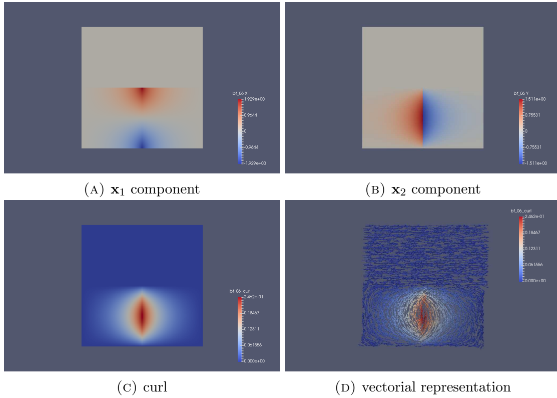
FIGURE 4. Edge shape function T\psi^6
