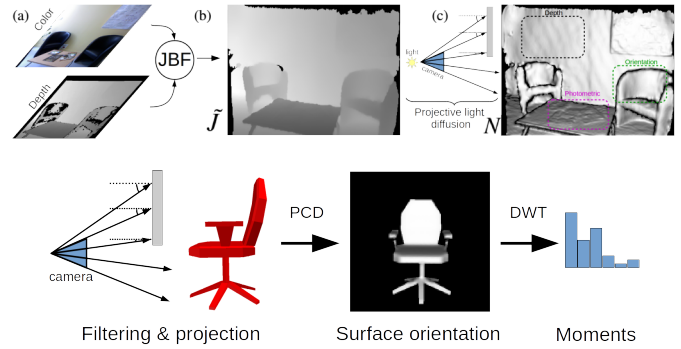
Fig. 4. PLDI on-line (first row) and off-line (second row) extraction pipelines.
