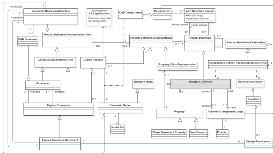
Fig. 3. KBE-PLM integration schema – CAD assembly models, CAD Design Intent, Design Rationale and Parameterization.
