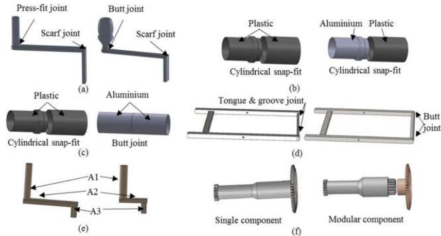
Fig. 2. (a) Change in joint design type (b) Change in material without change in joint design type (c) Change in material with change in joint design type (d) Change in component's dimension with change in joint design type (e) Change in component's dimension without change in joint design type (f) Change in product architecture
