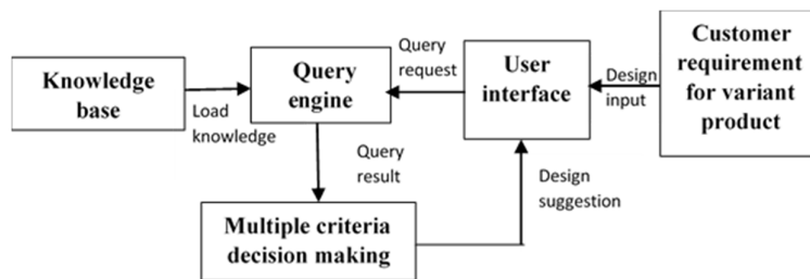
Fig. 1. Knowledge based framework for selection of joining process in variant design
