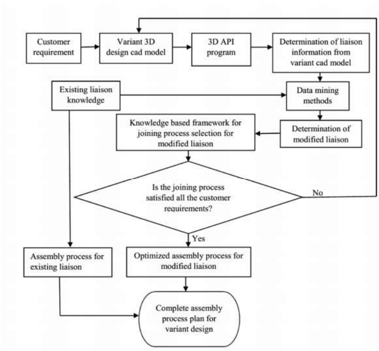
Fig. 5. A framework for variant design application
