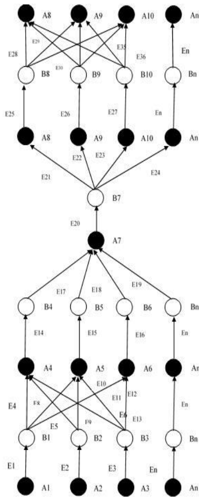
Fig. 2. Bi-graph Model of Supply chain process
