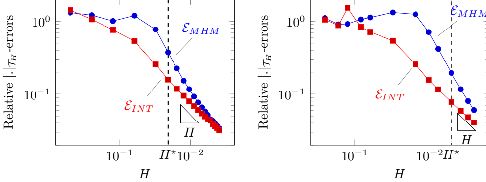
FIG. 6.2. Convergence curves for \ell = 0 with \omega = 20\pi (left) and \omega = 40\pi (right).
