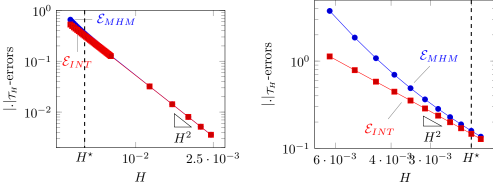
FIG. 6.3. Convergence curves for \ell = 1 with \omega = 30\pi (left) and \omega = 150\pi (right).
