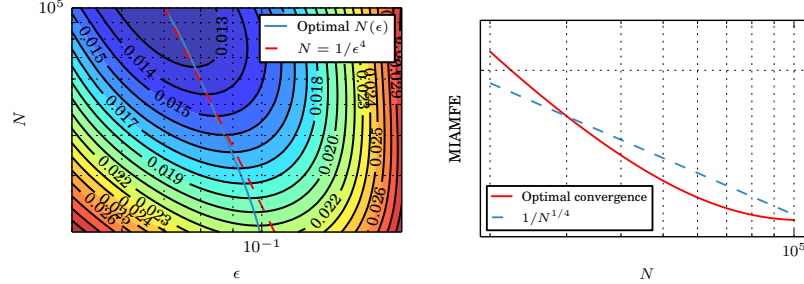
Fig. 1.6: L^1 error as a function \varepsilon and N . and optimal rate of convergence for the L^1 error
