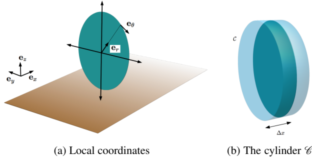
Fig. 1.9: Non rotating uniformly loaded actuator disc model. (a) The local reference frame at the actuator disc of the turbine, using cylindrical coordinates; (b) The cylinder \mathcal{C} that extends the actuator disc. Mill forces are applied to particles that lie inside.
