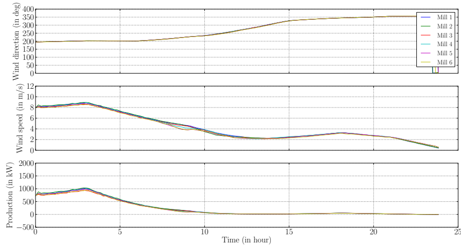
Fig. 1.12: Time evolution of SDM results for the 22 th December 2016
